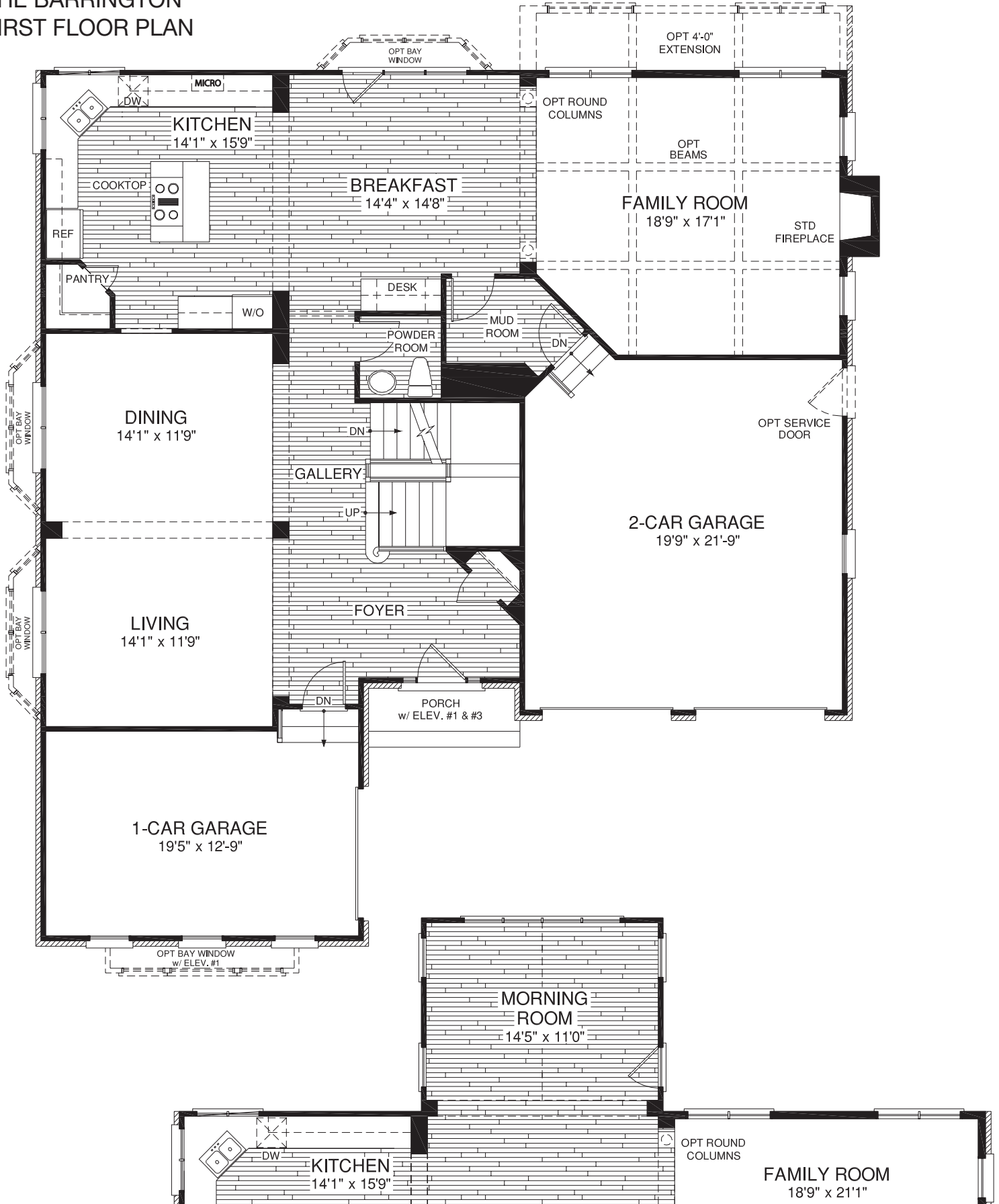
PARTIAL FIRST FLOOR w/ OPT MORNING ROOM
